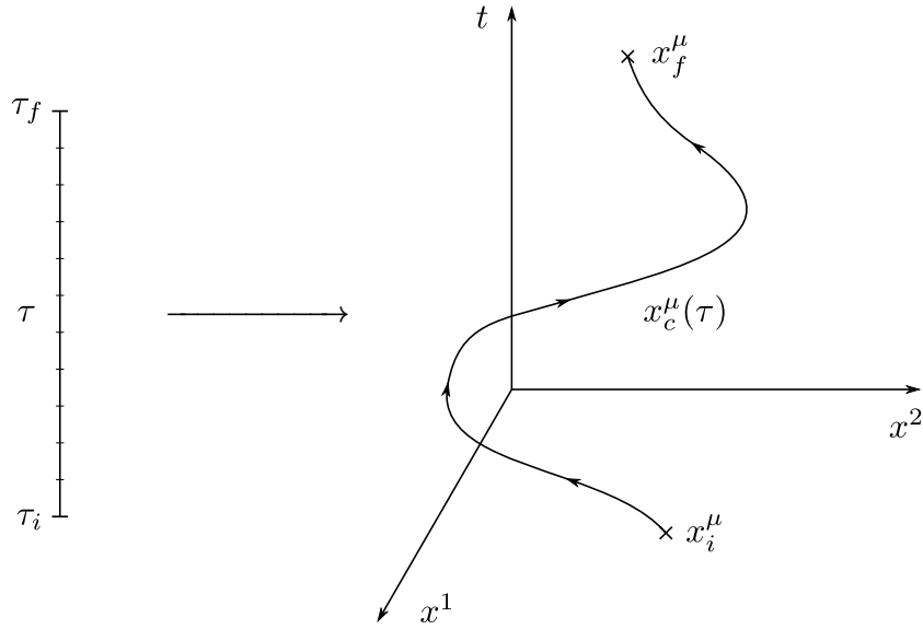
Figure 46.6: Trajectory x_c^\mu(\tau) of a particle in spacetime (worldline). The worldline is described by the parameter \tau \in [\tau_i, \tau_f] .
