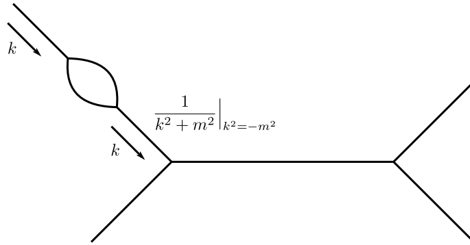
Figure 46.4: Due to the conservation of energy–momentum, the particle propagating after the loop is on-shell and this leads to a divergence of its propagator. This is cured by taking into account the mass renormalization and resummation of all the 1PR graphs.
