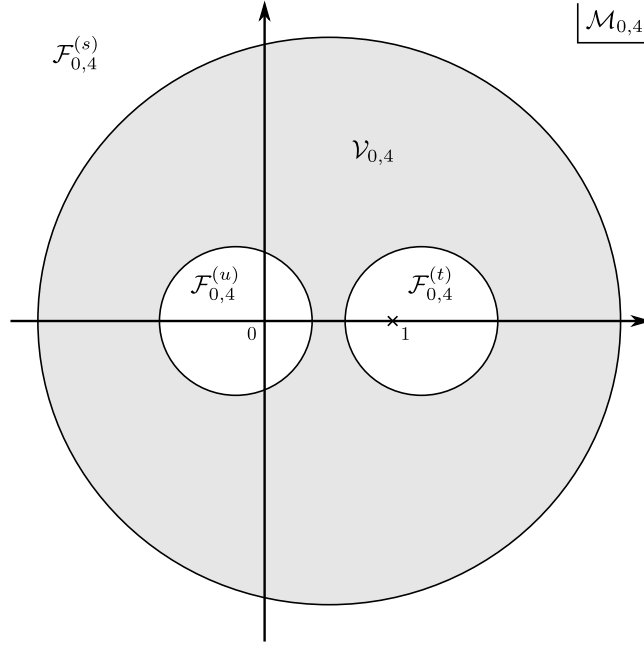
Figure 18.9: In white are the subspaces of the moduli space \mathcal{M}_{0,4} covered by the plumbing fixture. The three different regions correspond to the three different ways to pair the punctures (see Figure 18.7). In grey is the fundamental vertex region \mathcal{V}_{0,4} .
