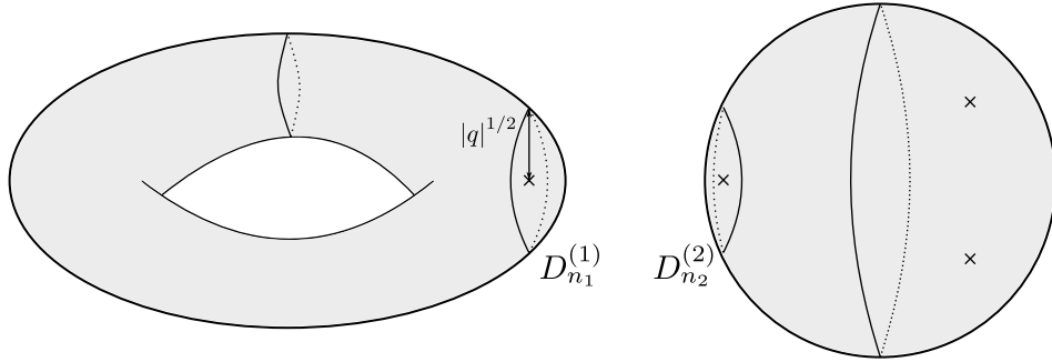
Figure 18.3: Disks around one puncture of the surfaces \Sigma_{1,1} and \Sigma_{0,3} . The disks appear as a cap because it is on top of the surface, which is curved.
