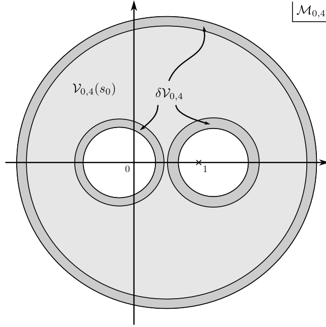
Figure 18.10: In light grey is the subspace covered by the \mathcal{V}_{0,4}(s_0) as in Figure 18.9. In dark grey is the difference \delta\mathcal{V}_{0,4} = \mathcal{V}_{0,4}(s_0 + \delta s_0) - \mathcal{V}_{0,4}(s_0) with \delta s_0 > 0 .
