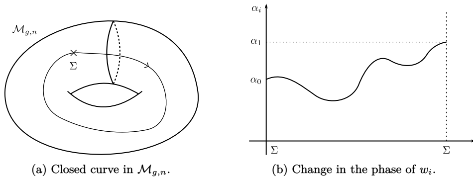
Figure 19.2: Schematic plot of the change in the phase of the local coordinate w_i as one follows a closed curve in \mathcal{M}_{g,n} . If the original phase at \Sigma is \alpha_0 and if the phase varies continuously along the path, then \alpha_1 \neq \alpha_0 when returning back to \Sigma by continuity.
