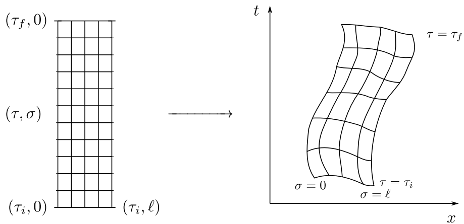
Figure 46.9: Trajectory x_c^\mu(\tau, \sigma) of an open string in spacetime (worldsheet). It begins and ends at the lines parametrized by x_i(\sigma) and x_f(\sigma) . The worldsheet is topologically a rectangle and is parametrized by (\tau, \sigma) \in [\tau_i, \tau_f] \times [0, \ell] .
