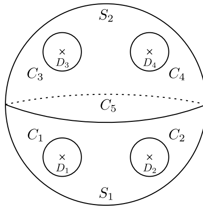
Figure 18.1: Parametrization of \Sigma_{0,4} .
