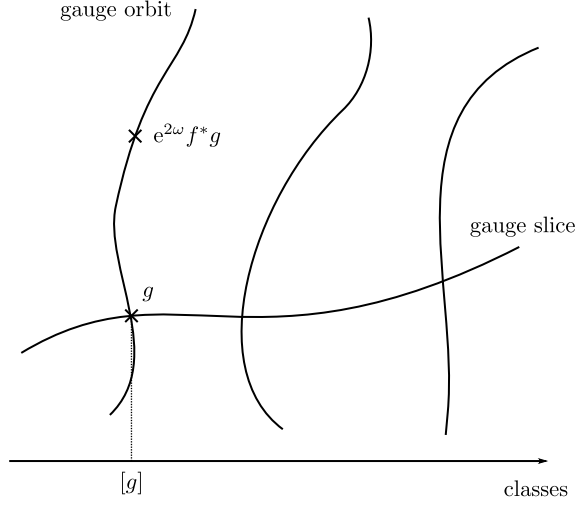
Figure 8.1: The space of metrics decomposed in gauge orbits. Two metrics related by a gauge transformation lie on the same orbit. Choosing a gauge slice amounts to pick one metric in each orbit, and the projection gives the space of metric classes.
