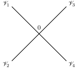
Figure 20.7: Fundamental quartic vertex.
