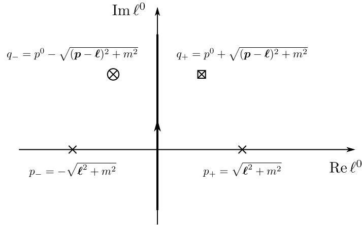
Figure 34.2: Integration contour for external Euclidean momenta.
