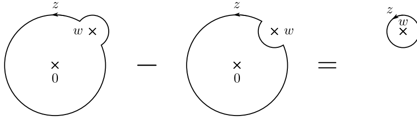
Figure 40.1: Graphical proof of (40.9).
