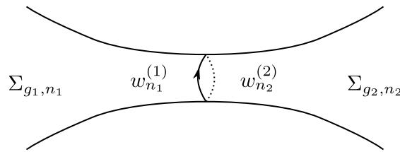
Figure 18.4: Integration contour on the circle between the two local coordinates which are glued together.
