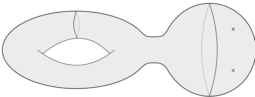
Figure 18.6: Smoothed connection between both surfaces.
