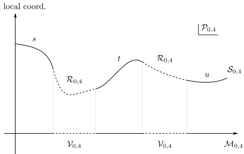
Figure 20.6: A section S_{0,4} over \mathcal{P}_{0,4} , the contribution from the s -, t - and u -channels (Figure 20.5) are indicated by the corresponding indices. The fundamental vertex is defined by the section \mathcal{V}_{0,4} .
