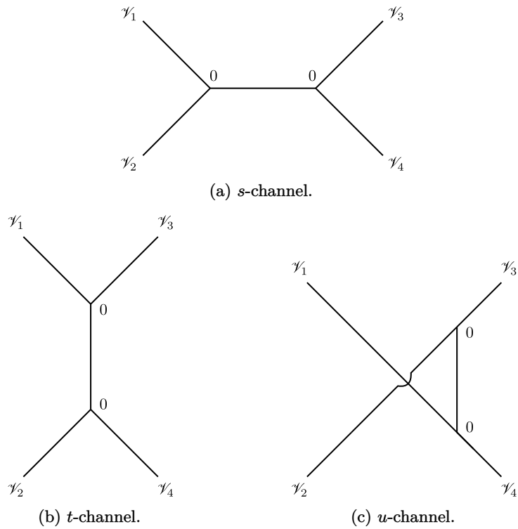
Figure 20.5: Factorization of the quartic amplitude A_{0,4} in the s -, t - and u -channels.
