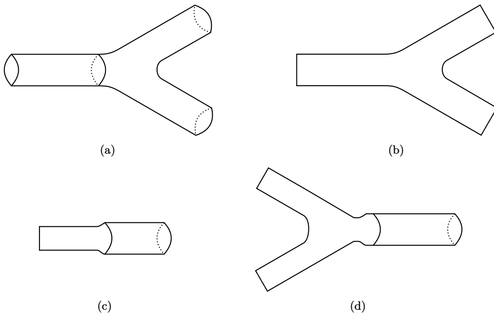
Figure 45.4: Worldsheet diagrams for string interactions.
