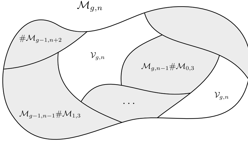
Figure 18.8: Schematic illustration of the covering of \mathcal{M}_{g,n} from the plumbing fixture of lower-dimensional spaces. The fundamental region \mathcal{V}_{g,n} (usually disconnected) is not covered by the plumbing fixture.
