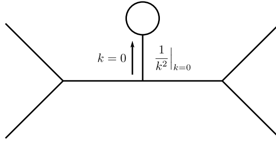
Figure 46.3: The momentum of the particle connecting the tadpole loop is forced to be zero due to the conservation of the energy–momentum. If the state is a massless particle, then it is on-shell and the propagator diverges. This means that the classical vacuum is destabilized and that there is a nearby vacuum with a lower energy.
