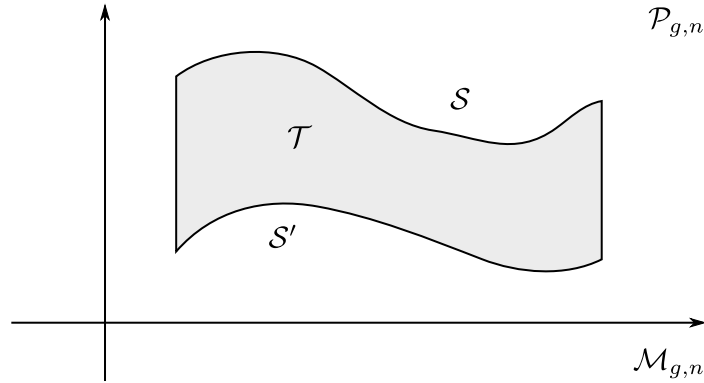
Figure 19.3: Two sections \mathcal{S} and \mathcal{S}' of \mathcal{P}_{g,n} delimiting a surface \mathcal{T} .
