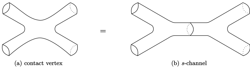
Figure 45.5: Scattering of four closed strings. Due to the non-locality the process on the left is equivalent to the one of the right, where an intermediate string propagates. The s -channel is displayed.
