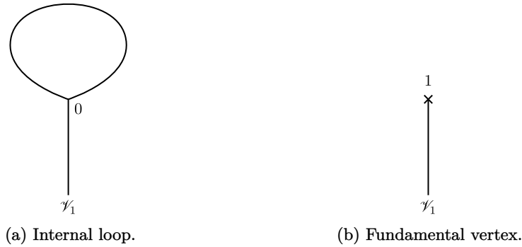
Figure 20.9: Factorization of the amplitude G_{1,1} and fundamental tadpole at 1-loop.
