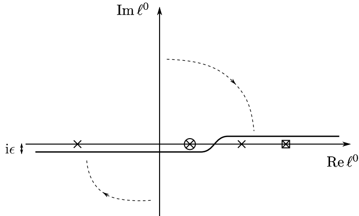
Figure 34.3: Integration contour for external Lorentzian momenta after Wick rotation (regular vertices).
