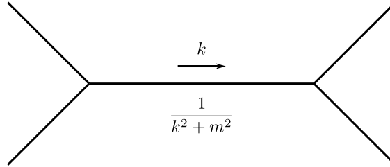
Figure 46.5: The amplitude diverges when the external momenta are such that k becomes on-shell. Physically, the internal particle is stable at the classical level, which is in contradiction with its decay, and hence the divergence. Quantum effects give an imaginary part to the mass, indicating that the particle can decay.
