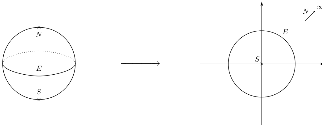
Figure 39.1: Map from the Riemann sphere to the complex plane. The south and north poles are denoted by the letter S and N , and the equatorial circle by E .
