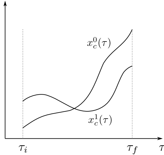
Figure 46.7: Examples of values for x^\mu(\tau) (note that x^0 is monotonically increasing).
