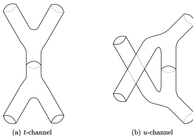
Figure 45.6: Scattering of four closed strings through the t - and u -channels.
