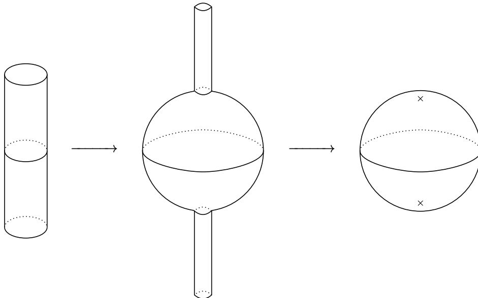
Figure 39.2: Map from the cylinder to the sphere with two tubes, to the 2-punctured sphere \Sigma_{0,2} .
