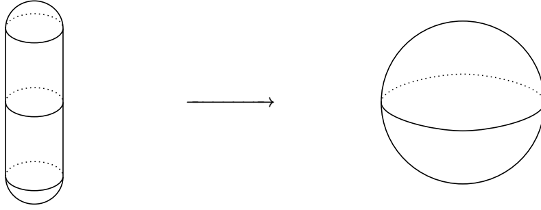
Figure 39.3: Map from the cylinder with two caps (half-spheres) to the Riemann sphere \Sigma_0 .
