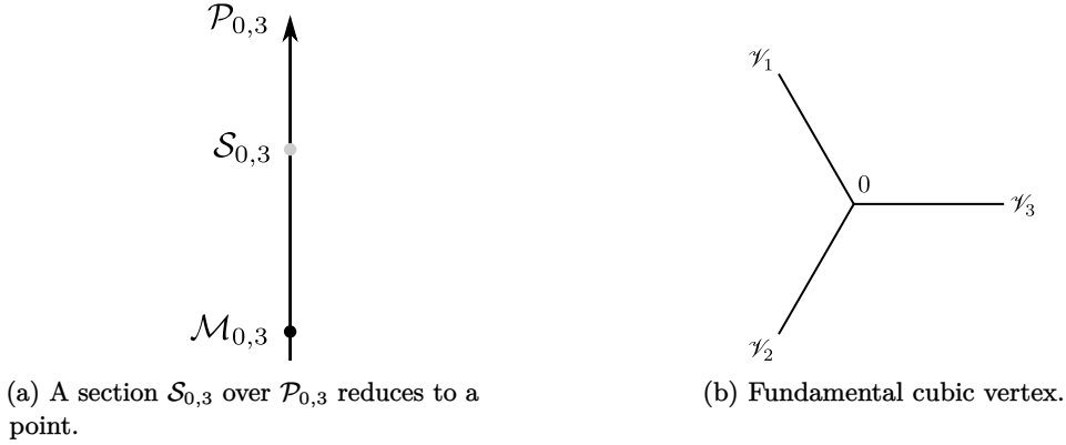
Figure 20.4: Section of \mathcal{P}_{0,3} and cubic vertex.
