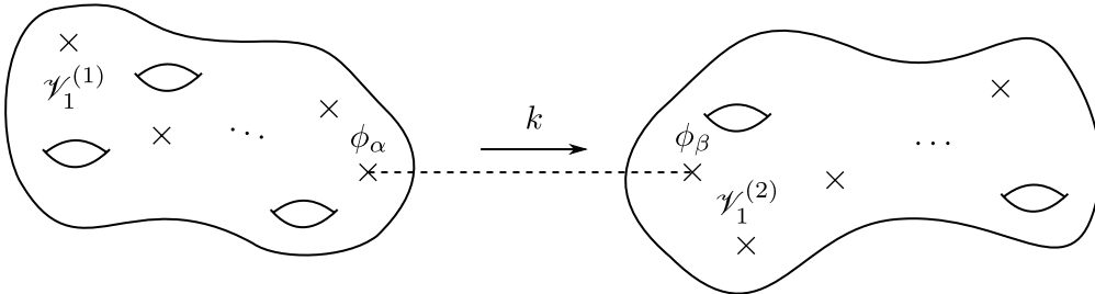
Figure 20.2: Factorization of the amplitude into two sub-amplitudes connected by a propagator (dashed line).
