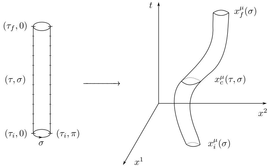
Figure 46.8: Trajectory x_c^\mu(\tau, \sigma) of a closed string in spacetime (worldsheet). It begins and ends at the circles parametrized by x_i(\sigma) and x_f(\sigma) . The worldsheet is topologically a cylinder and is parametrized by (\tau, \sigma) \in [\tau_i, \tau_f] \times [0, 2\pi) .
