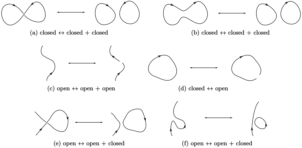
Figure 45.1: Joining and splitting of oriented strings. All these processes are oriented because one can consistently draw an arrow on each diagram before and after the interactions.
