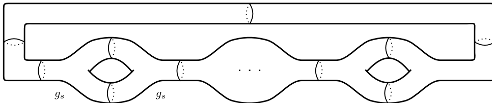
Figure 8.2: g -loop partition function.
