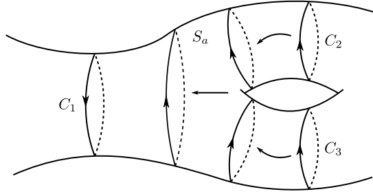
Figure 19.1: Deformation of the contour of integration defining the Beltrami form for a reparametrization of z_a . The figure is drawn for two circles at a hole, but the proof is identical for other types of circles.
