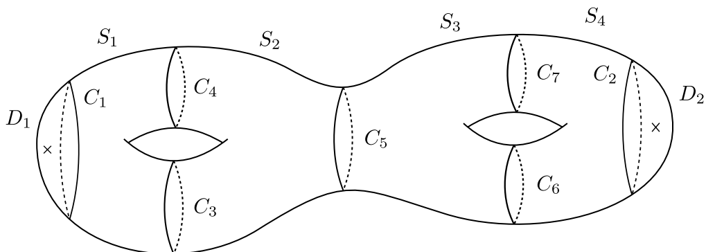
Figure 18.2: Parametrization of \Sigma_{2,2} .
