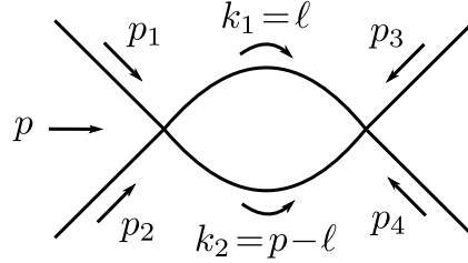
Figure 34.1: 1-loop 4-point function for a scalar field theory.
