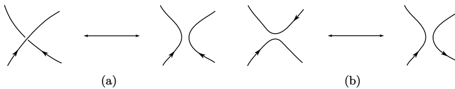
Figure 45.3: Recombinations of two open strings into two strings.
