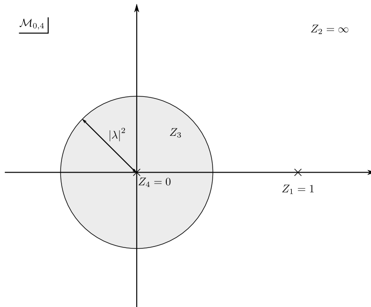
Figure 21.1: Part of the moduli space \mathcal{M}_{0,4} = \mathbb{C} (parametrized by Z_3 ) covered by the s -channel graph.
