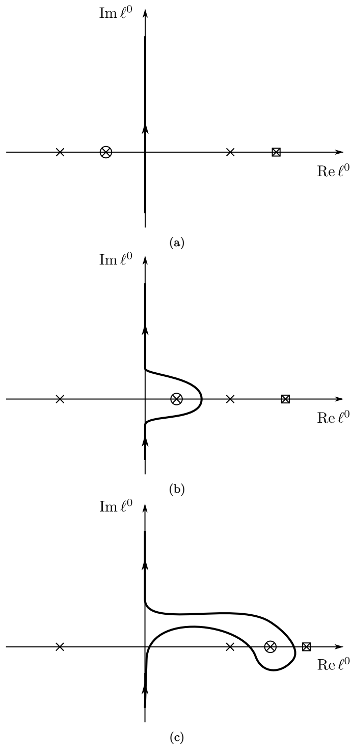
Figure 34.4: Integration contour after analytic continuation to external Lorentzian momenta. Depending on the values of the external momenta, different cases can happen.
