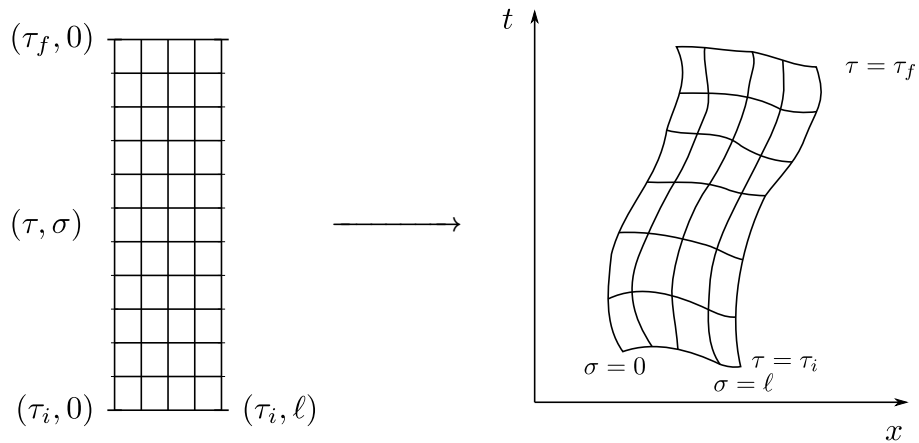
Figure 1.5: Trajectory x_c^\mu(\tau, \sigma) of an open string in spacetime (worldsheet). It begins and ends at the lines parametrized by x_i(\sigma) and x_f(\sigma) . The worldsheet is topologically a rectangle and is parametrized by (\tau, \sigma) \in [\tau_i, \tau_f] \times [0, \ell] .
