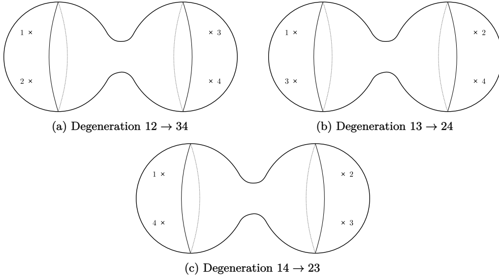
Figure 18.7: Permutations of punctures while gluing two spheres: they correspond to different (disconnected) parts of \mathcal{M}_{0,4} .
