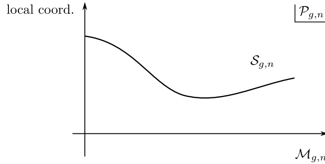
Figure 17.2: Section \mathcal{S}_{g,n} of the fibre bundle \mathcal{P}_{g,n} , the latter having \mathcal{M}_{g,n} as a base the local coordinates as a fibre.
