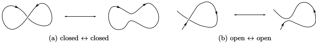
Figure 45.2: Joining and splitting of unoriented strings. These two processes are non-oriented because part of the string should flip its orientation during the interaction.
